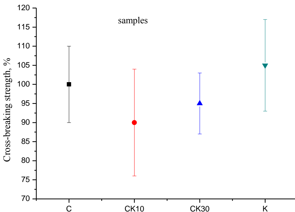
Dependence of the cross-breaking strength on the pellets composition
