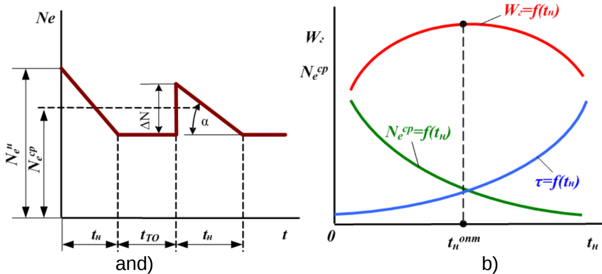
Fig. 1. Power change (a), and performance parameters affecting it (b), depending on the length of the machine ( t_h ) And the duration of maintenance ( t_{TO} )
