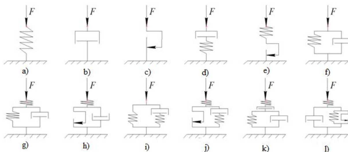
Fig. 1. The main rheological models, where F - external force: a - Hooke; b - Newton; c - Saint-Wenan; d - Maxwell; e - Prandtl; f - Voigt; g - Kelvin; h - Binham; i - Poynting-Thomson; j - Shvedov; k - Burgers; l - Imlinskiy.
