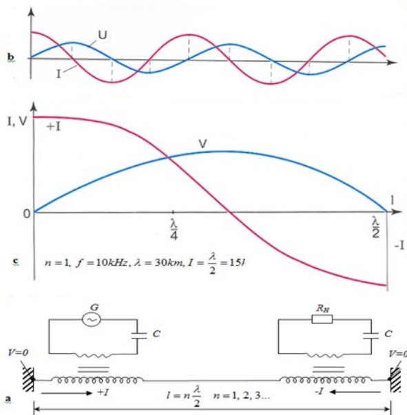
Fig. 5. Current and voltage distribution in a single-conductor line shorted to the ground at both ends: a – circuit representation ( G – high-frequency generator, R_H – load resistance, C – capacitance of the resonant circuit); b – current and voltage standing wave distribution along a single-conductor line; c – current and voltage distribution in a half-wave single-conductor line.
