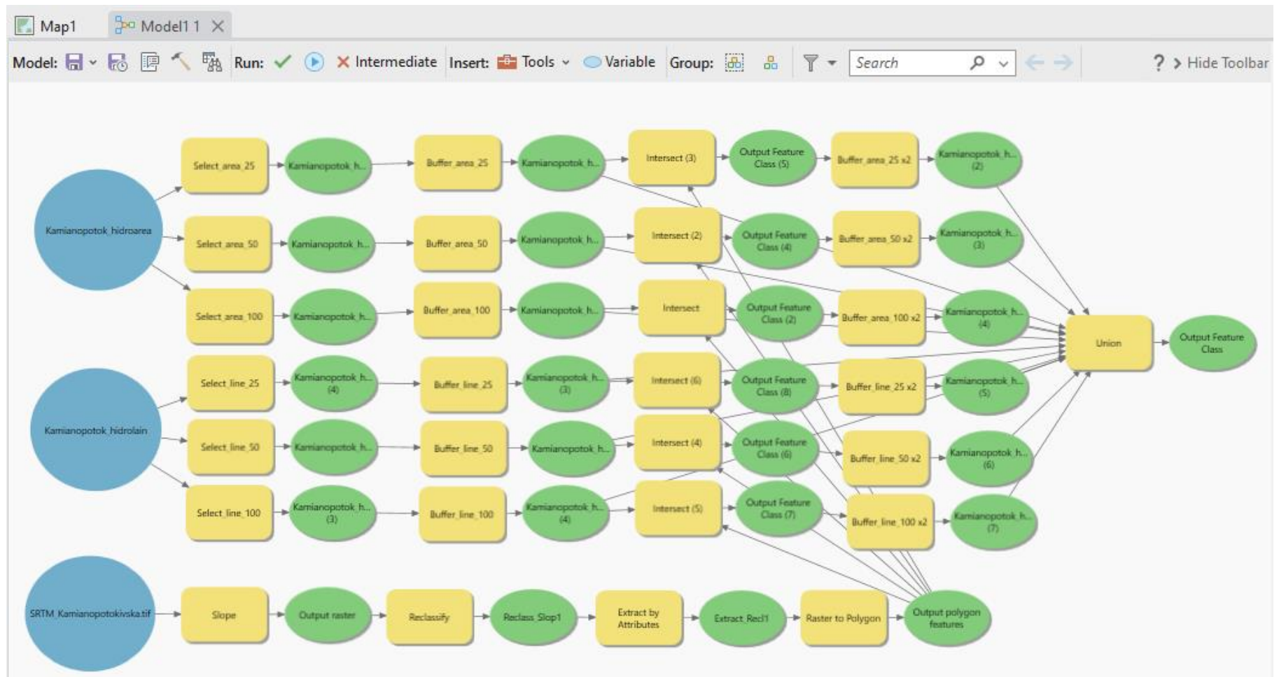
Fig. 1 Final automated model for designing coastal protection strips of water protection zones
